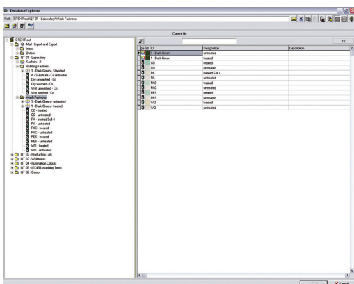
Database explorer
